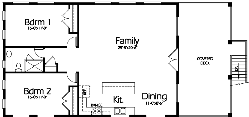
Upper Level 1380 Sq. Feet
